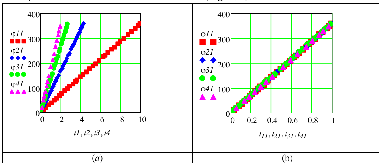
Fig. 2. Dimensional (a) and dimensionless (b) change in time of the law of motion of the input half-coupling for different values of the number of revolutions of the input link. Symbols \blacksquare ; \blacklozenge ; \bullet and \blacktriangle corresponds to the number of rotation of the input link, respectively equal to 6; fourteen; 22 and 30 rpm values.
