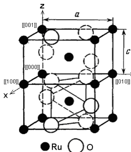
3-rasm. RuO 2 ning elementar yacheykasi
